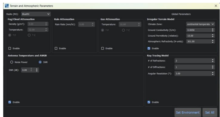
setup Terrain and Atmospheric parameters
