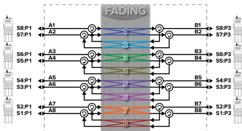
MESH Radio Network for Radios with Dual-Antenna
